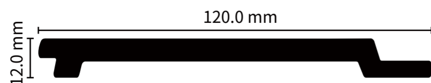
ITEM NO.: PG-12012-10 SIZE: 120x12MM LENGTH: 2.9M
