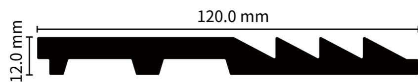
ITEM NO.: PG-12012-4 SIZE: 120x12MM LENGTH: 2.9M
