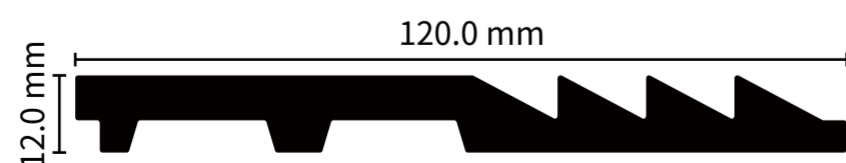
ITEM NO.: PG-12012-5 SIZE: 120x12MM LENGTH: 2.9M
