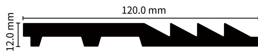
ITEM NO.: PG-12012-2 SIZE: 120x12MM LENGTH: 2.9M
