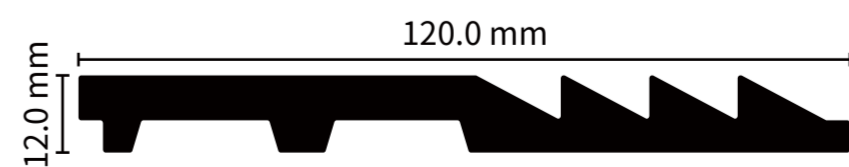
ITEM NO.: PG-12012-11 SIZE: 120x12MM LENGTH: 2.9M
