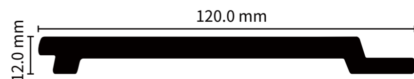
ITEM NO.: PG-12012-9 SIZE: 120x12MM LENGTH: 2.9M
