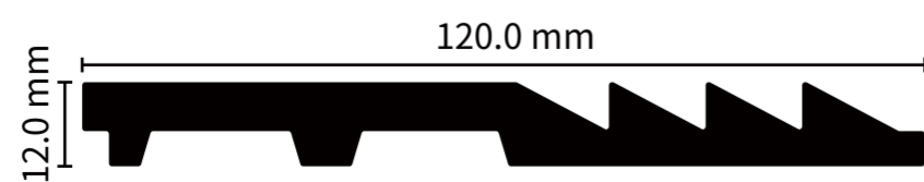
ITEM NO.: PG-12012-13 SIZE: 120x12MM LENGTH: 2.9M
