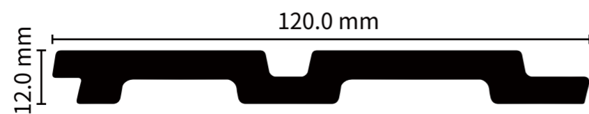
ITEM NO.: PG-12012-8 SIZE: 120x12MM LENGTH: 2.9M
