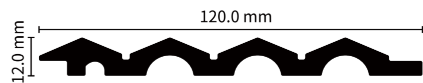
ITEM NO.: PG12012-14 SIZE: 120x12MM LENGTH: 2.9M
